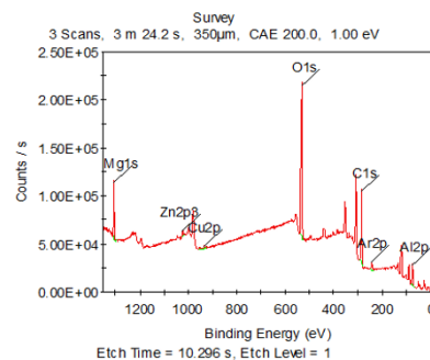
Figure 8. Typical survey scan for AA7075-T73 aluminum alloy
