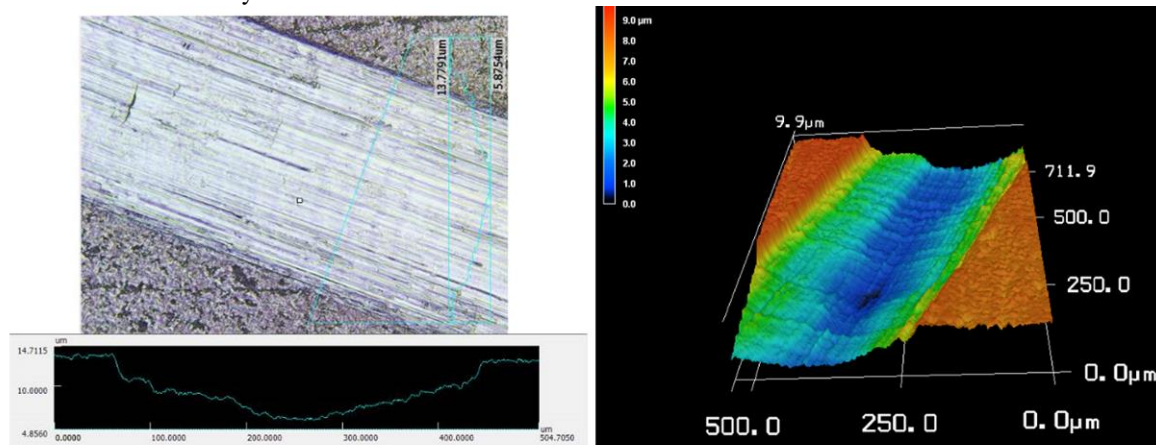
Figure 7. Cylindrical carbide scribe profile imaged using laser confocal microscopy.
