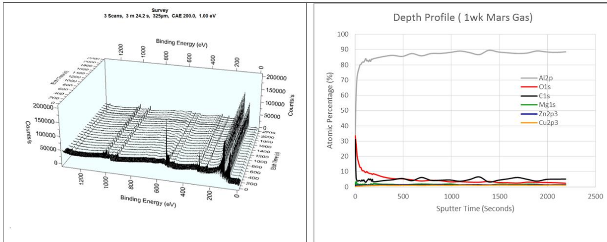
Figure 17. Survey scan and depth profile data collected over the scribed area of an AA7075-T73 alloy sample exposed to Mars Gas for one week at a temperature of 20°C and a pressure of 700 Pa.
