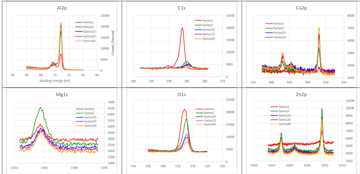
Figure 16. Selected spectra of individual element scans from the depth profile data collected over the scribed area of an AA7075-T73 alloy sample exposed to CO 2 for one week at 20°C and a pressure of 700 Pa.
