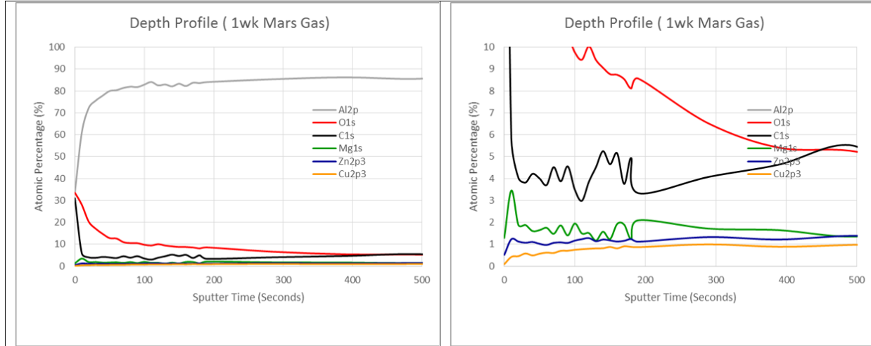
Figure 18. Depth profile data collected over the scribed area of an AA7075-T73 alloy sample, immediately after exposure to Mars gas for one week, zoomed in for 0-500 seconds etch time (left image) and for 0-10 atomic percentage (right image).
