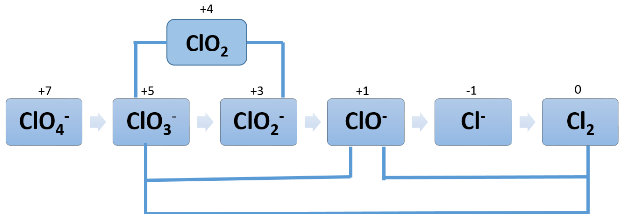
Figure 3. Oxidation state diagram for oxychlorine species.
