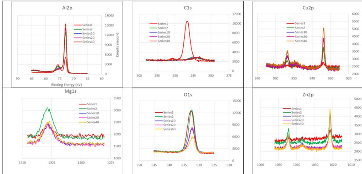
Figure 11. Selected spectra of individual element scans from the depth profile of AA7075-T73 control sample (minimal exposure to air of the scribed area).
