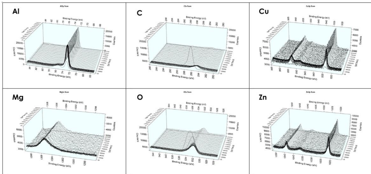
Figure 15. Depth profile data, for individual elements, collected over the scribed area of an AA7075-T73 alloy exposed to CO 2 for one week at room temperature and a pressure of 700 Pa.
