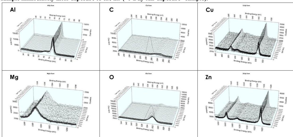
Figure 10. Depth profile data, for individual elements, collected over the scribed area of an AA7075-T73 aluminum alloy sample immediately after exposure to the air (“0-Day-Air exposure” sample).
