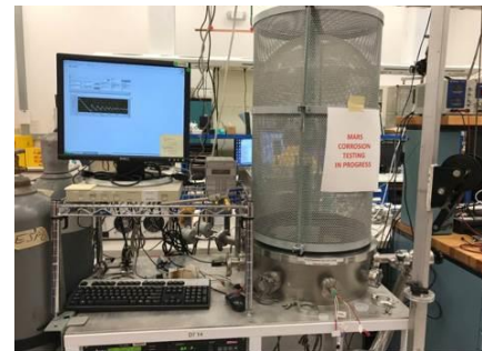
Figure 4. Mars chamber at KSC.
