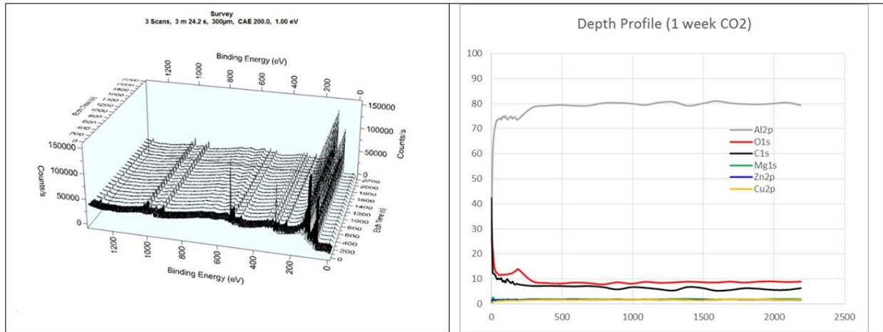
Figure 13. Survey scan and depth profile data collected over the scribed area of an AA7075-T73 alloy sample exposed to CO 2 for one week at 700 Pa (7 mbar) pressure and room temperature.
