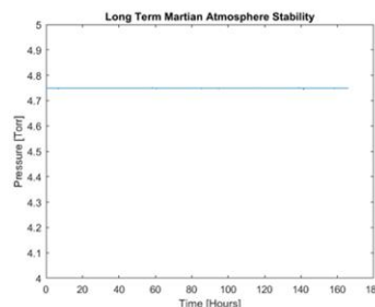
Figure 5. Pressure data from a representative long-term exposure experiment inside the Mars chamber (1 Torr = 0.133 kPa).
