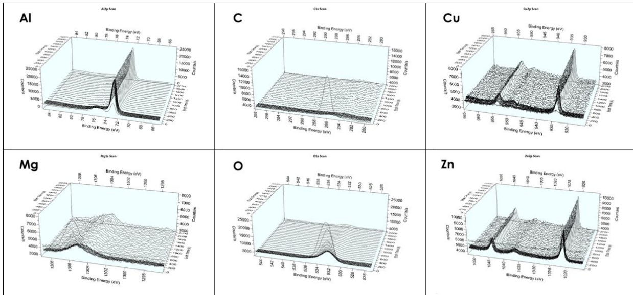
Figure 19. Depth profile data, for individual elements, collected over the scribed area of an AA7075-T73 alloy exposed to Mars gas for one week at a temperature of 20°C and a pressure of 700 Pa.
