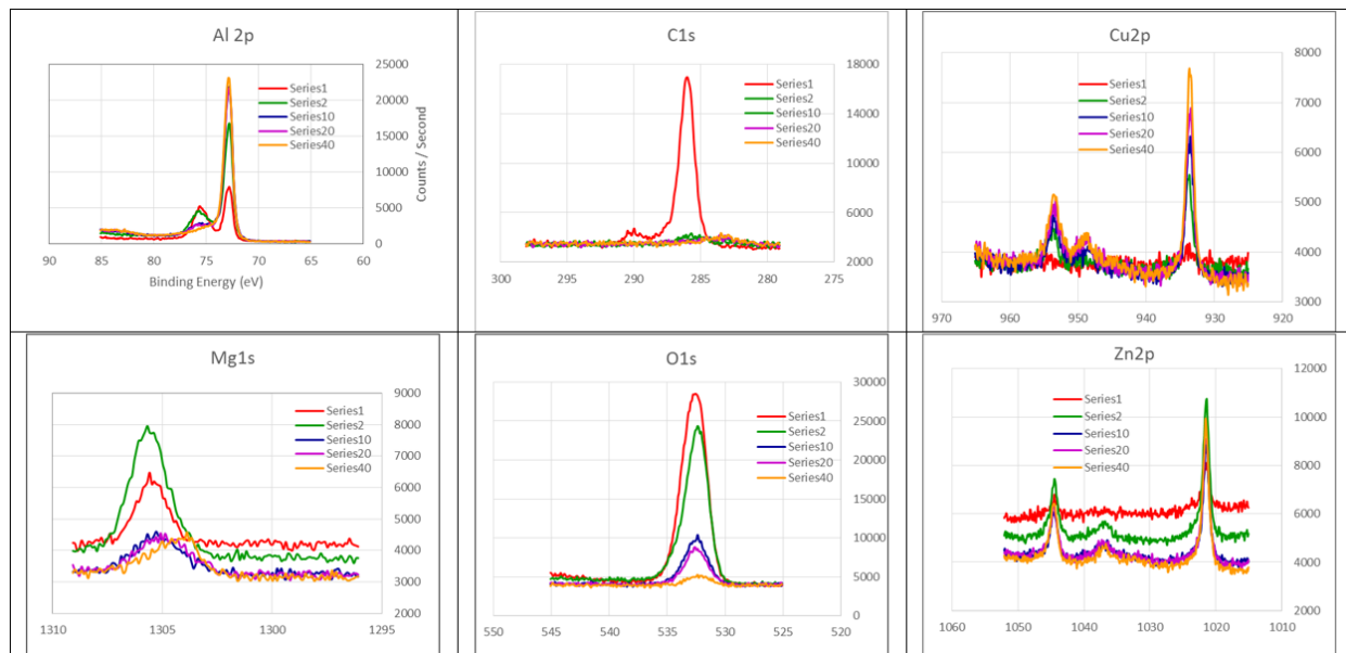
Figure 20. Selected spectra of individual element scans from the depth profile data collected over the scribed area of an AA7075-T73 alloy sample exposed to Mars gas for one week at room temperature and a pressure of 700 Pa (7 mbar).
