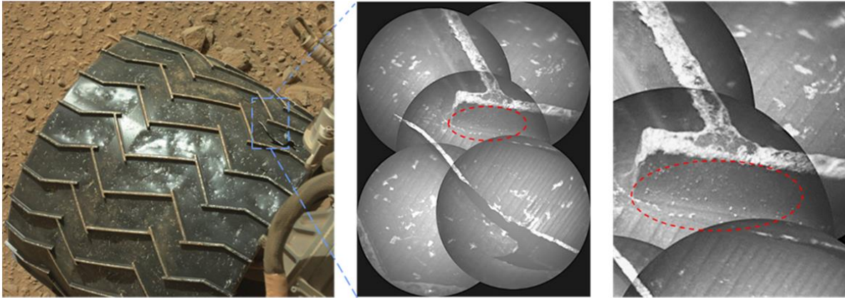
Figure 2. Curiosity's ChemCam images of a damaged area of the rover's middle right-wheel. The image shows not only a large crack in the wheel (area inside blue rectangle on left image) but some sub-millimeter-sized blisters in the vertical wall of the T-print of the wheels (circled in red on the middle and right images) which cannot be attributed to rock scratching. It has been suggested that the blisters are caused by the corrosive interaction between transient brines and the aluminum alloy.
