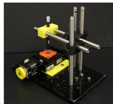
Figure 6. Sample holder with scribing tool.
