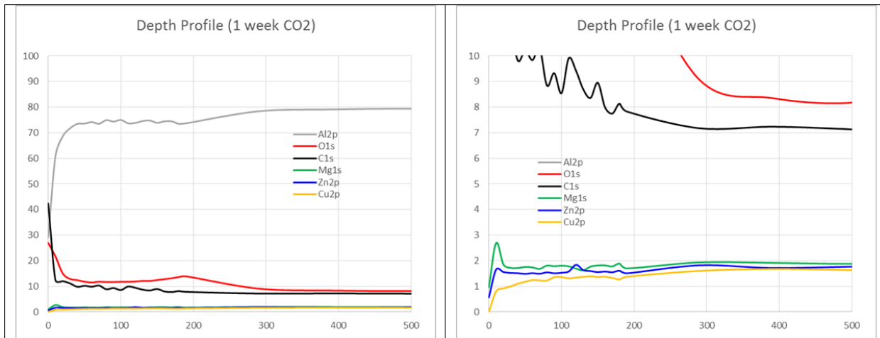
Figure 14. Depth profile data collected over the scribed area of an AA7075-T73 aluminum alloy sample, immediately after exposure to CO 2 for one week, zoomed in for 0-500 seconds etch time (left image) and for 0-10 atomic percentage (right image).
