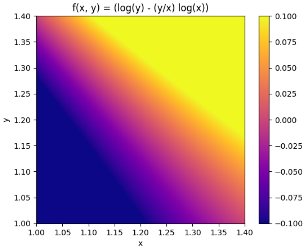
FIGURE 1. Plot of the function f(x, y) = (\log(y) - \frac{y}{x} \cdot \log(x)) .
