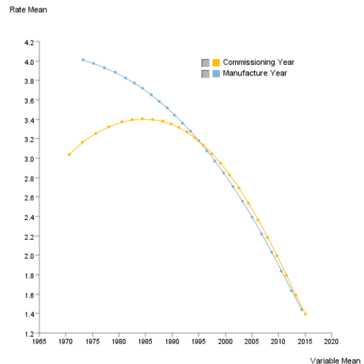
Fig. 11. Naive Bayes model correlation between Commissioning and Manufacturing year with the leak rate.
