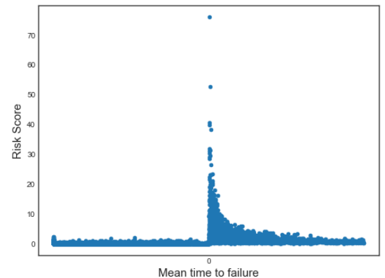
Fig. 1. Risk factor calculated by XGBoost for each item as function of the MTTF (negative values represent censored data).
