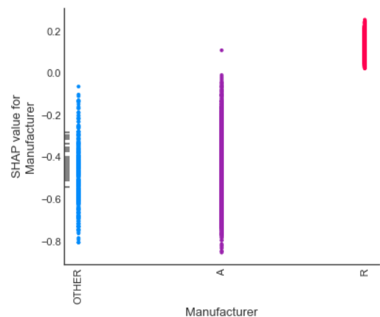
Fig. 4. SHAP dependence plot, showing how the model output varies by the manufacturer value.
