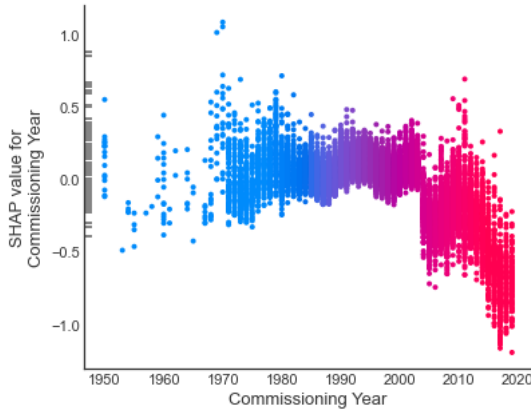
Fig. 6. SHAP dependence plot, showing how the model output varies by the commissioning year value.
