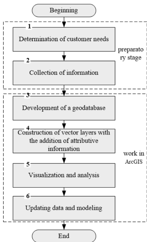
Fig. 4. GIS design algorithm for monitoring
