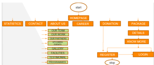
Figure 1. Data flow diagram
